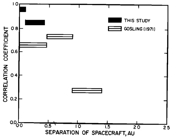
Fig. 3. The correlation coefficient of corotation pairs of velocity measurements as a function of the distance between two spacecraft. The correlation coefficients from this study (solid bars) and from Gosling [1971] (open bars) are shown. The separation between the spacecraft in Gosling's study was mainly azimuthal (see text).
