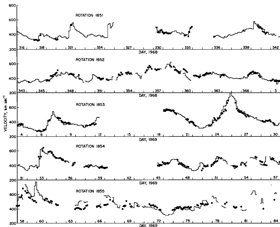
Fig. 2. The 3-hour averages of the solar wind velocity observed at Pioneer 9 (bars) and at Ogo 5 (circles) as a function of time at Pioneer 9. The Ogo 5 data were translated to Pioneer 9 time by using the 3-hour average of the velocity at Pioneer 9 and the corotation model (see text).
