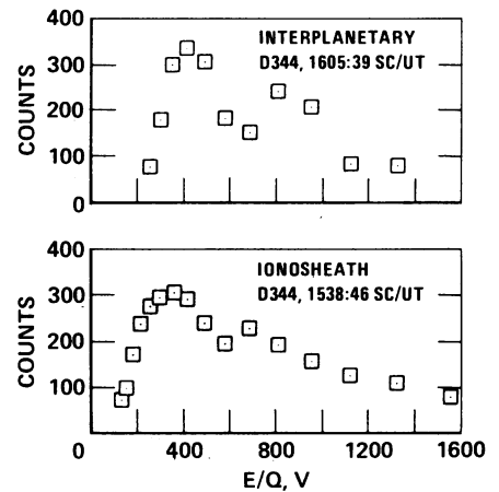
Fig. 1 (left). Daily solar wind proton peak speeds measured during December 1978. In most cases, the data were obtained near noon universal time for each orbit, upstream from the bow shock. Fig. 2 (right). Comparison of ionosheath and interplanetary ion spectra across the bow shock during the outbound leg of orbit 6. The parameters derived from these spectra by a Maxwellian fit are, for the interplanetary case, v = 287 km/sec, N = 33 \text{ cm}^{-3} , and T = 20,700 K; and for the ionosheath case; v = 254 km/sec, N = 87 \text{ cm}^{-3} , and T = 67,000 K.
