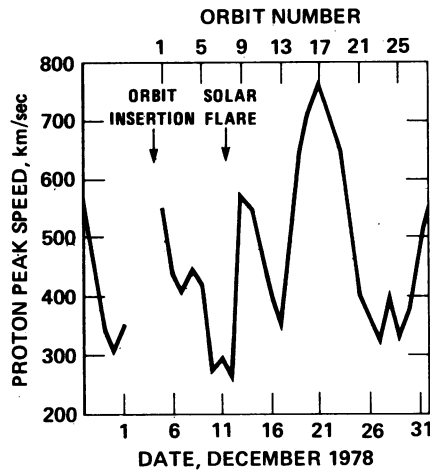
Fig. 1 (left). Daily solar wind proton peak speeds measured during December 1978. In most cases, the data were obtained near noon universal time for each orbit, upstream from the bow shock. Fig. 2 (right). Comparison of ionosheath and interplanetary ion spectra across the bow shock during the outbound leg of orbit 6. The parameters derived from these spectra by a Maxwellian fit are, for the interplanetary case, v = 287 km/sec, N = 33 \text{ cm}^{-3} , and T = 20,700 K; and for the ionosheath case; v = 254 km/sec, N = 87 \text{ cm}^{-3} , and T = 67,000 K.
